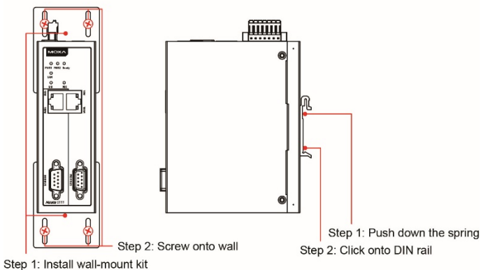
Wall-Mount Installation
